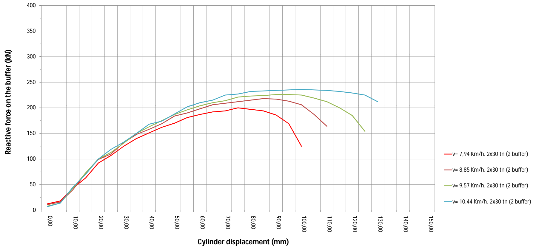
Force-displacement for a impact of 2 masses of 30tn (2 buffers) at different velocities
